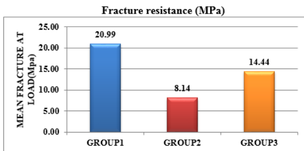
Fig. 2: Mean fracture resistance of three groups.
