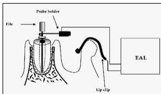
Fig. 1: Circuit for electronic determination of working length
